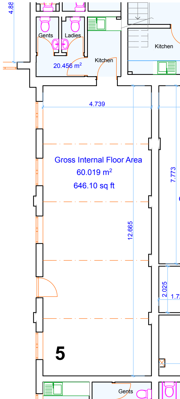
0. Ground Floor 1:100
